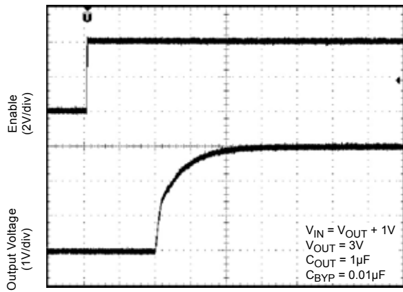
Time (10µs/div)
