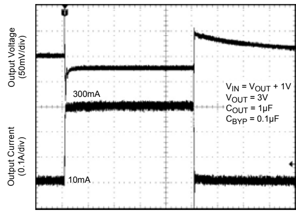
Time (20µs/div)
